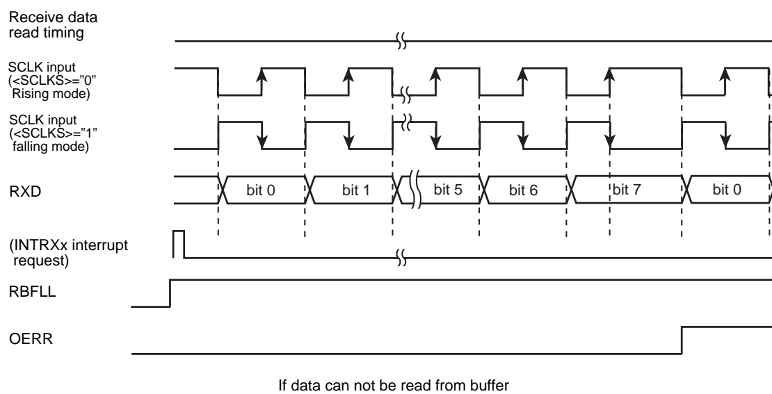
Figure 12-15 Receive Operation in the I/O Interface Mode (SCLK Input Mode)
