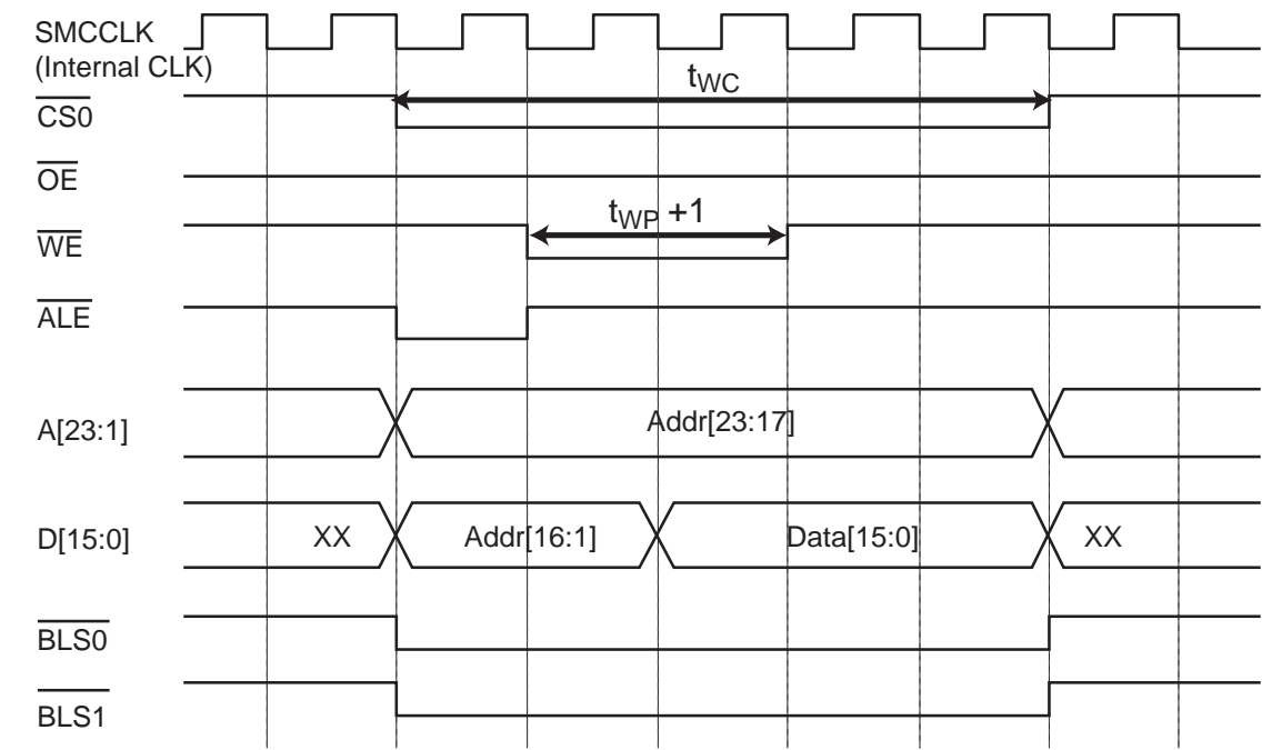
Figure 10-7 Asynchronous Write
